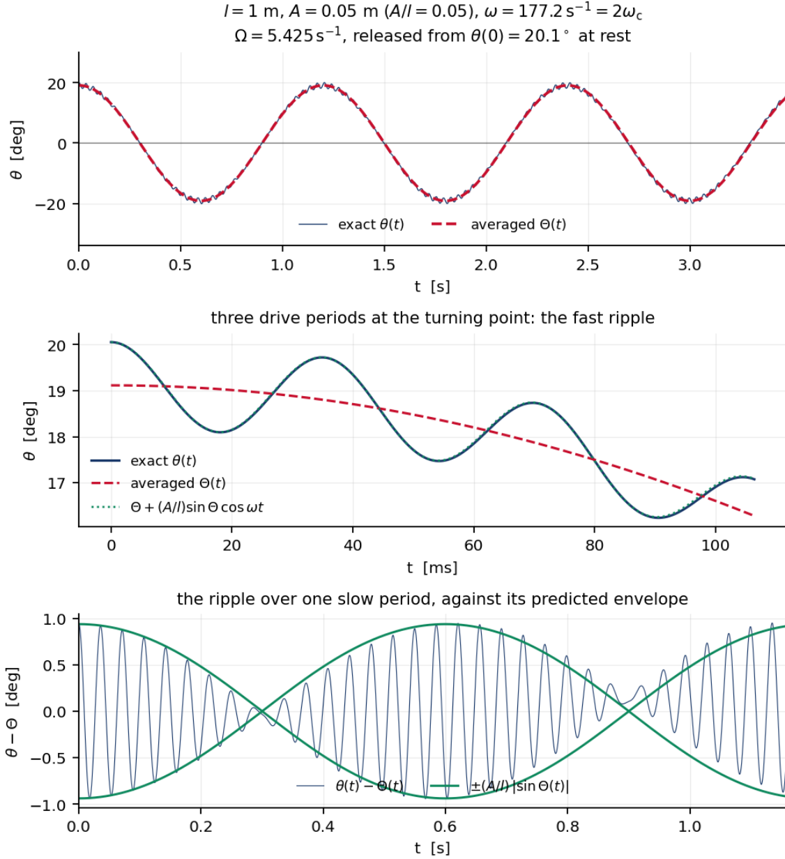
Figure 1. l = 1 \text{ m}, A = 0.05 \text{ m}, \omega = 2\omega_c = 177.2 \text{ s}^{-1} , released from \theta(0) = 20.1^\circ at rest. Top: the exact solution of (16) and the averaged solution of (28), over three slow periods. Middle: three drive periods at the turning point, where the ripple is largest; the dotted curve is \Theta + \varepsilon \sin \Theta \cos \omega t from (24) and is indistinguishable from the exact solution at this scale. Bottom: the residual \theta - \Theta over one slow period against the predicted envelope \pm \varepsilon |\sin \Theta| , showing the ripple collapsing to zero each time the pendulum passes through the vertical, which is the signature of the \sin \Theta factor in (24).
